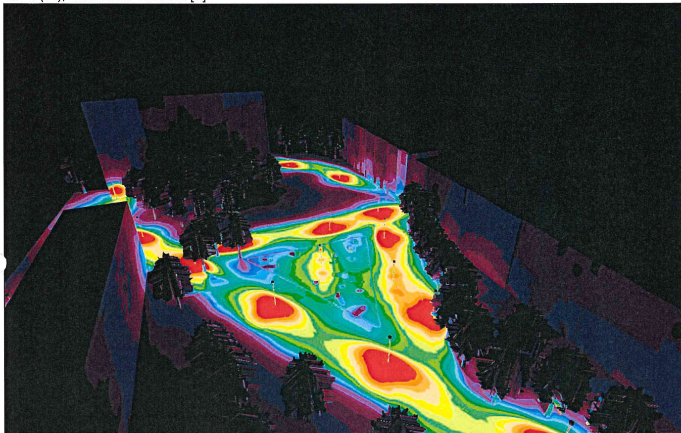
Site 1 (51), Illuminance values in [lx]
