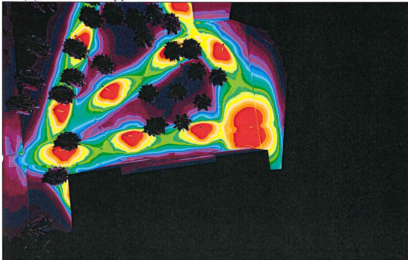
Site 1 (57), Illuminance values in [lx]
