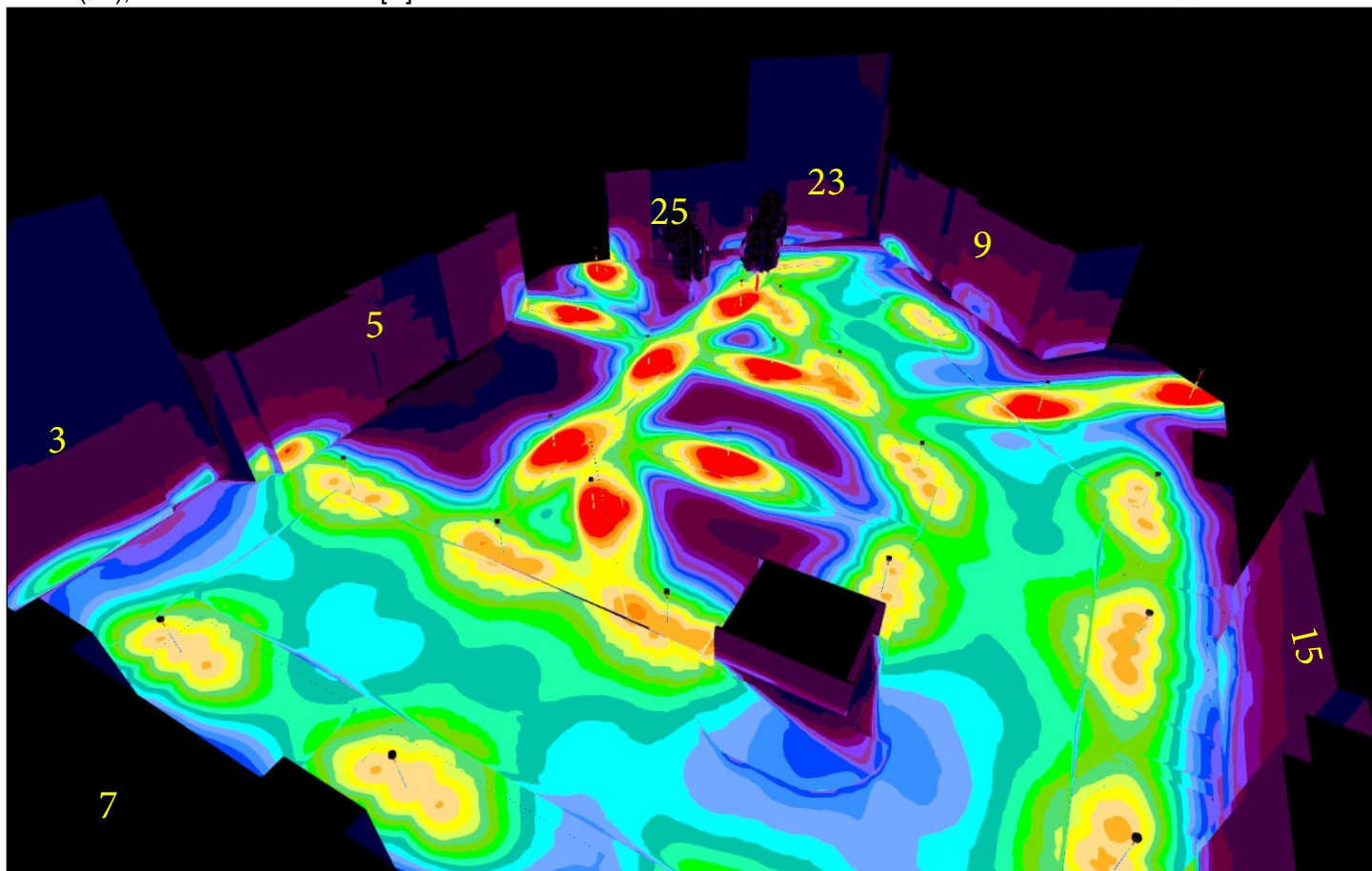
Site 1 (80), Illuminance values in [lx]
