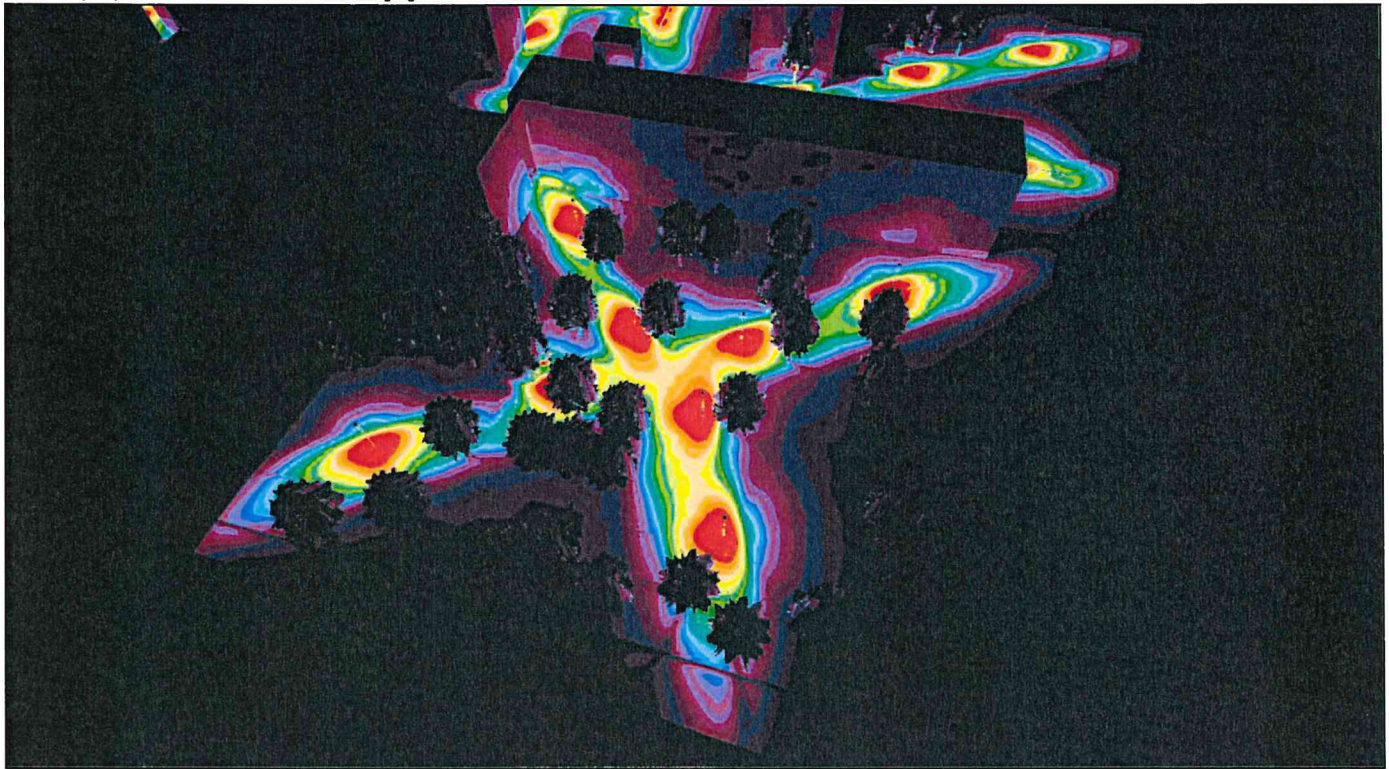
Site 1 (23), Illuminance values in [lx]
