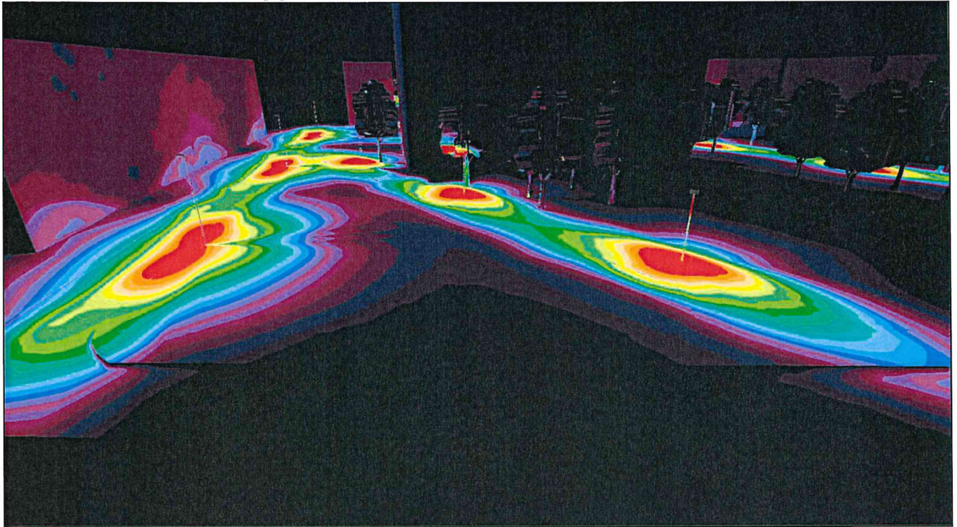
Site 1 (27), Illuminance values in [lx]
