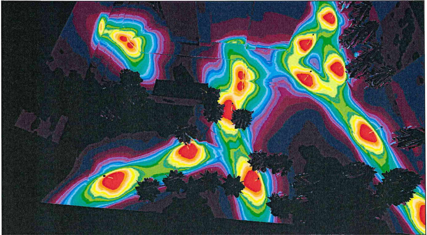
Site 1 (39), Illuminance values in [lx]
