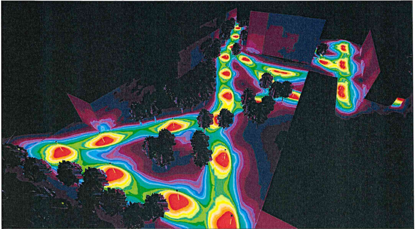
Site 1 (31), Illuminance values in [lx]
