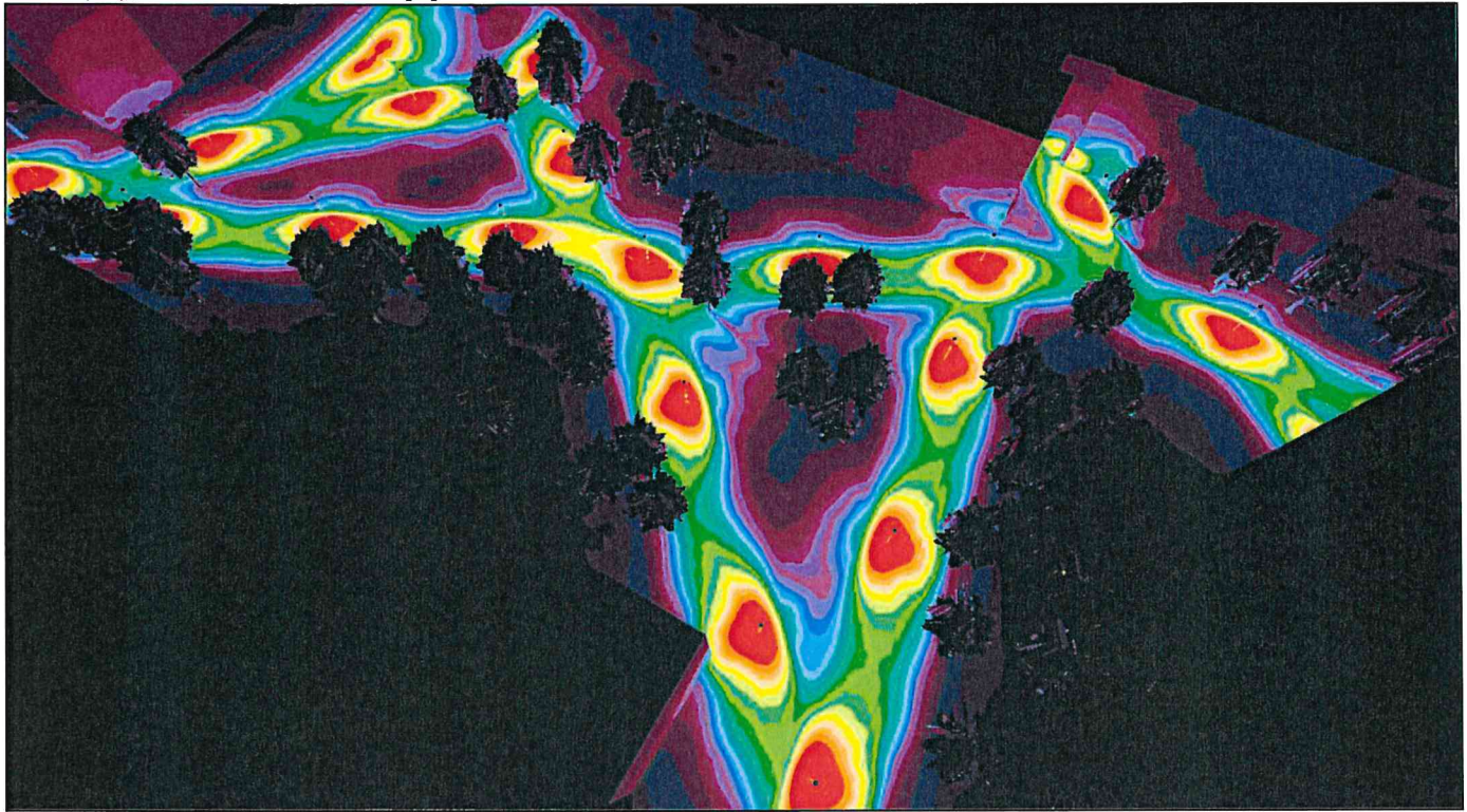
Site 1 (33), Illuminance values in [lx]
