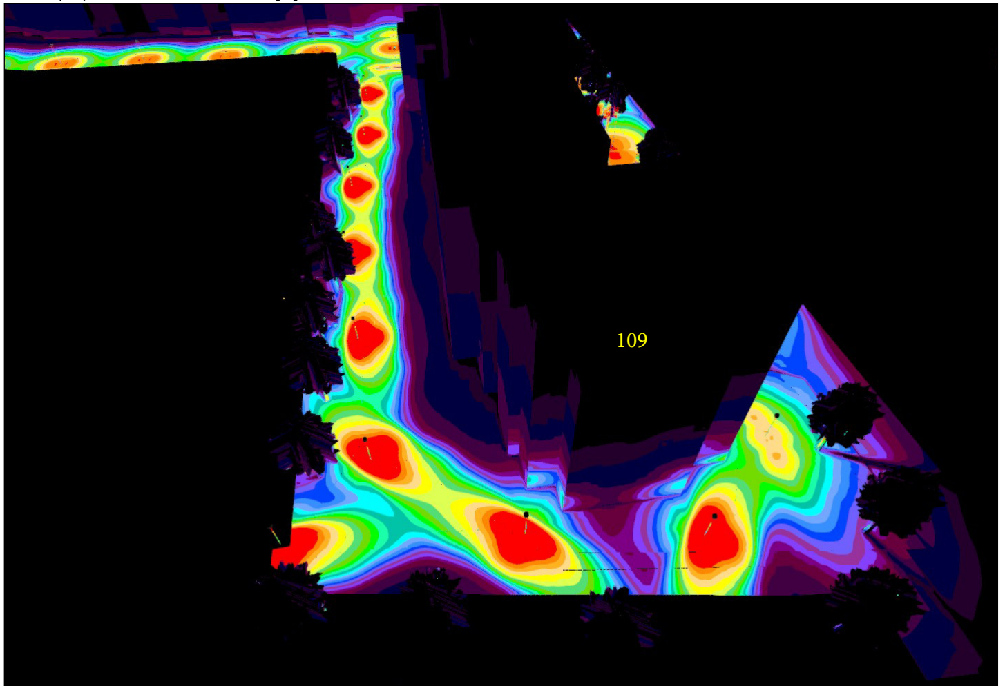
Site 1 (43), Illuminance values in [lx]
