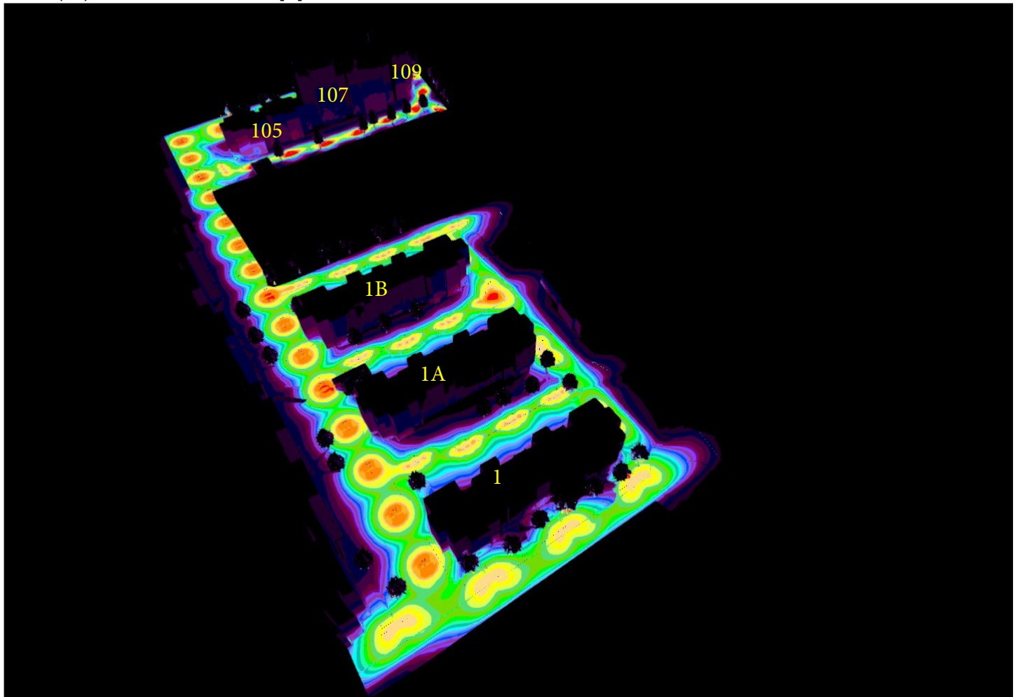
Site 1 (63), Illuminance values in [lx]
