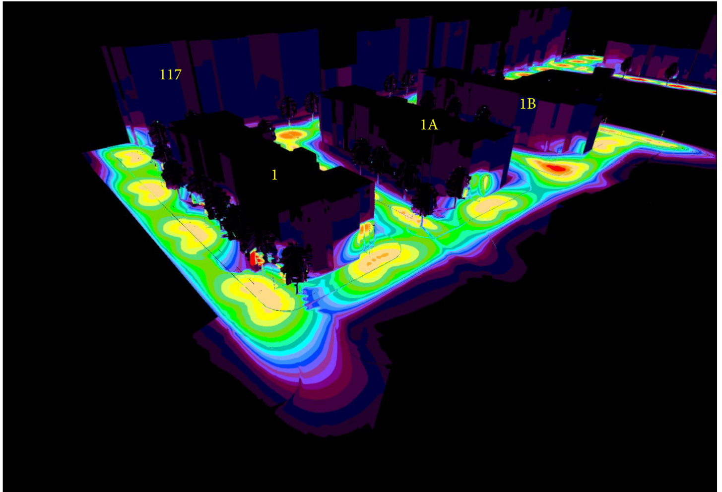
Site 1 (35), Illuminance values in [lx]
