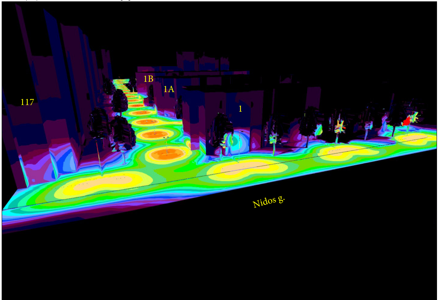
Site 1 (59), Illuminance values in [lx]
