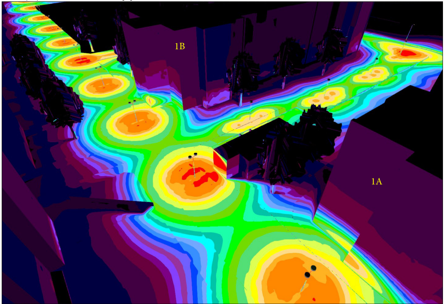
Site 1 (53), Illuminance values in [lx]
