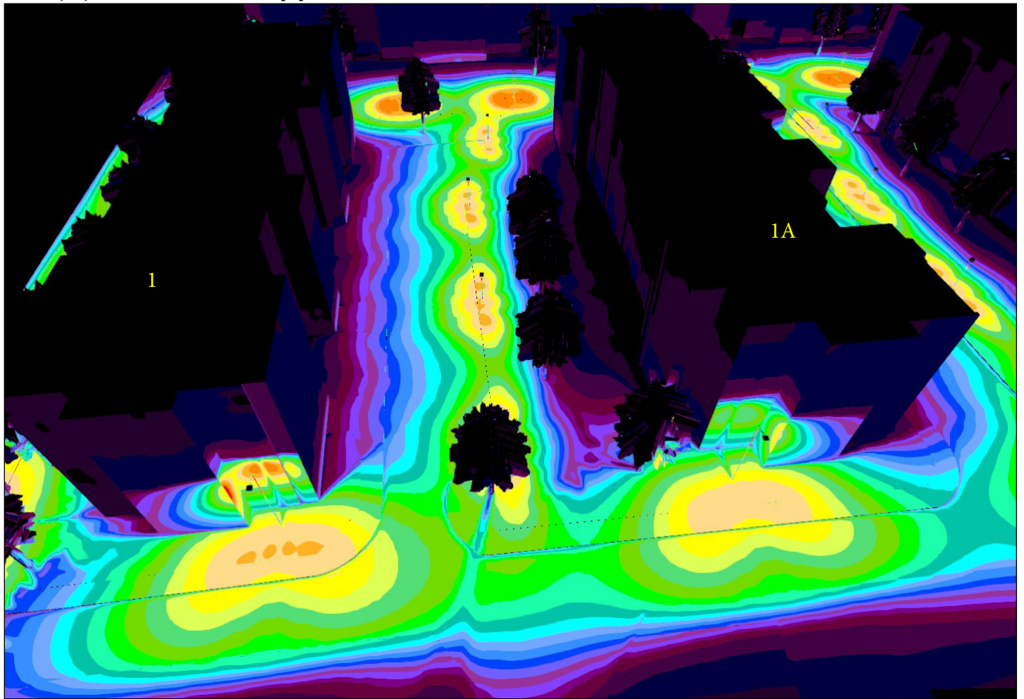
Site 1 (37), Illuminance values in [lx]
