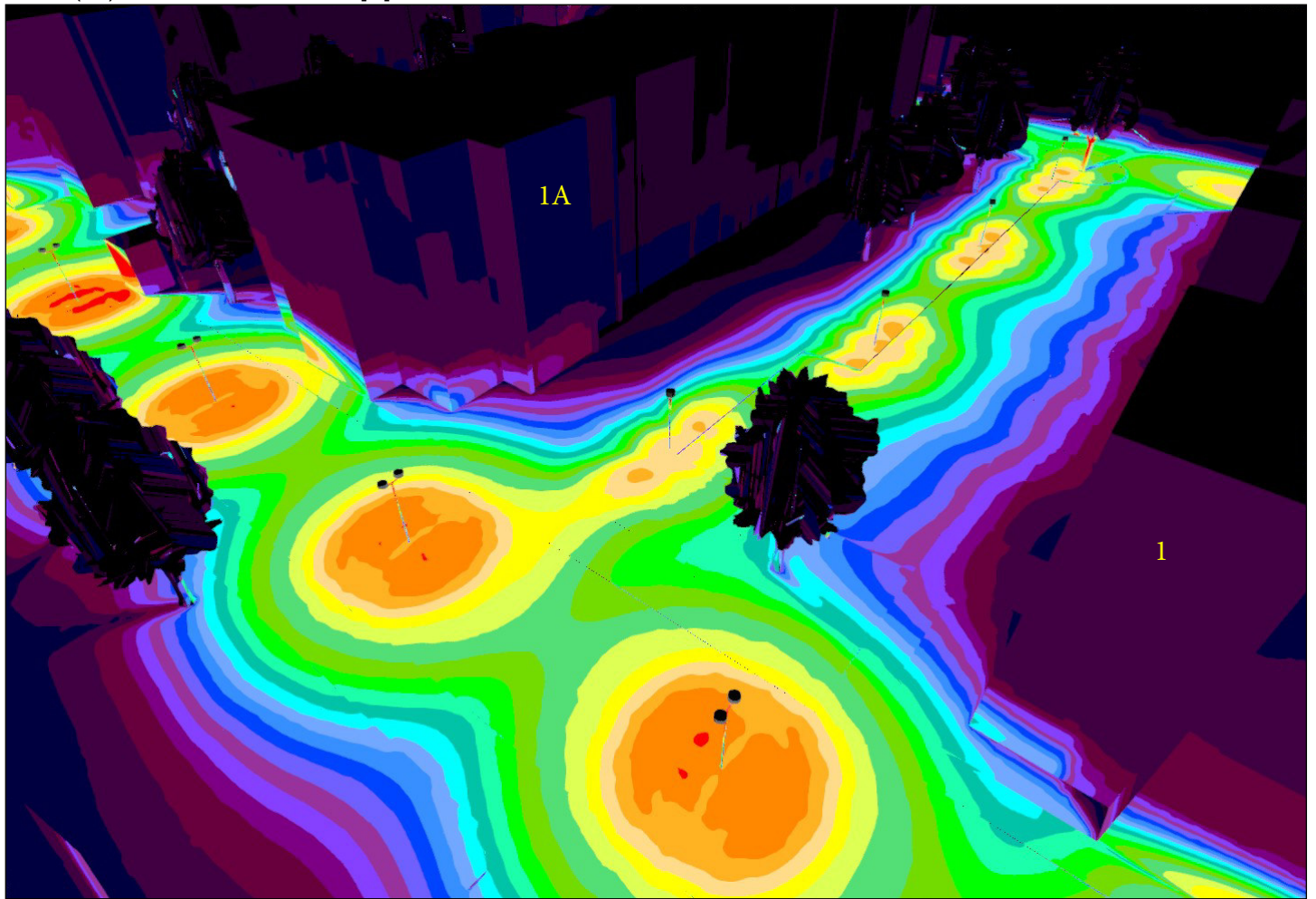
Site 1 (57), Illuminance values in [lx]
