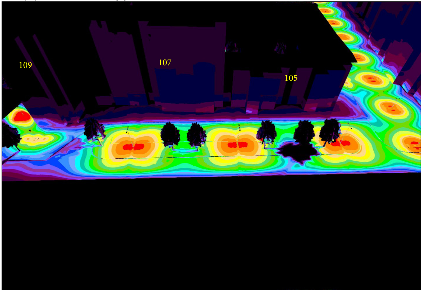
Site 1 (45), Illuminance values in [lx]
