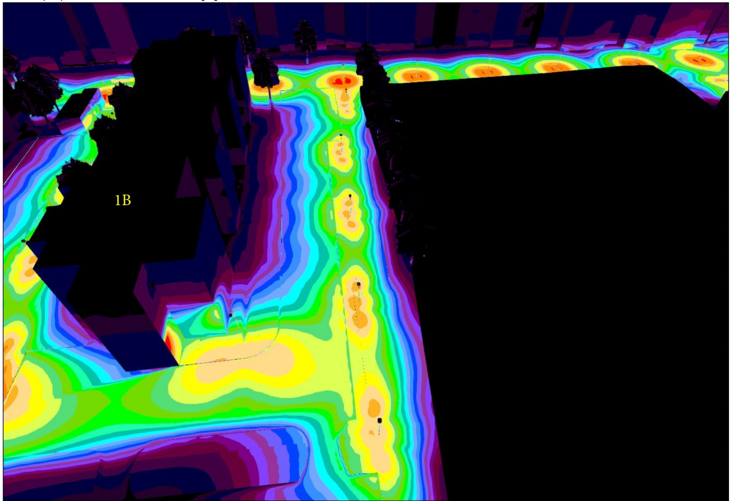
Site 1 (41), Illuminance values in [lx]
