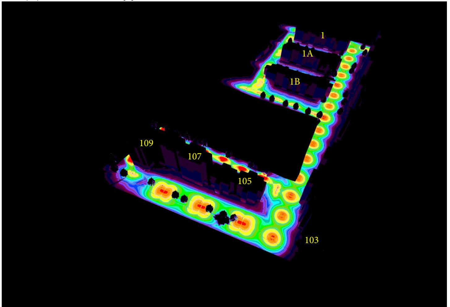
Site 1 (65), Illuminance values in [lx]
