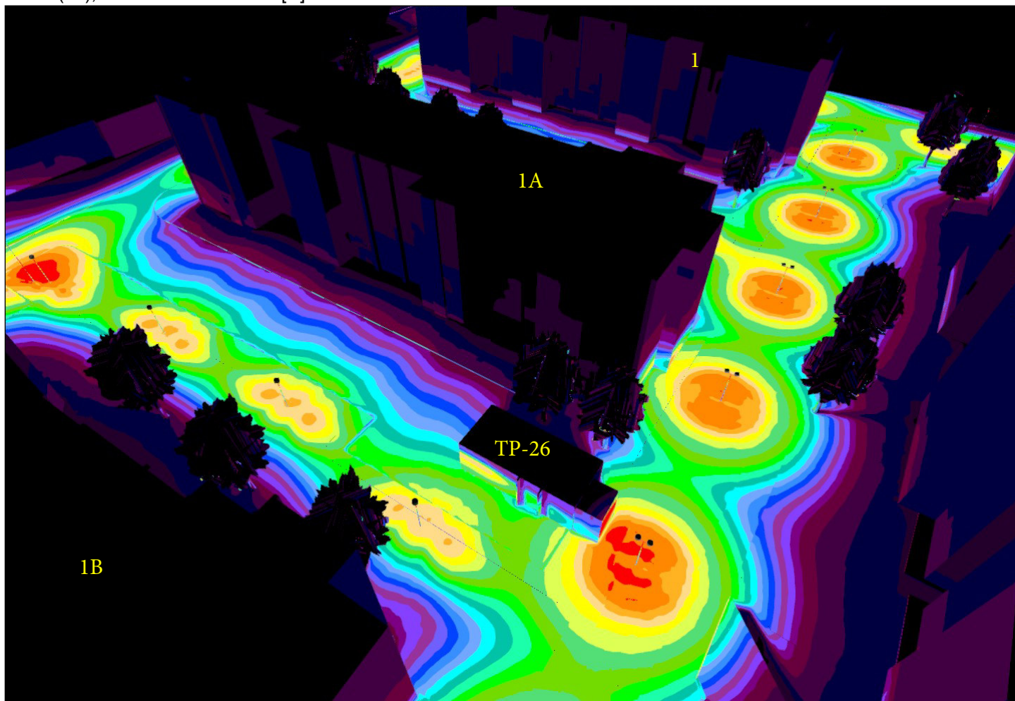
Site 1 (55), Illuminance values in [lx]
