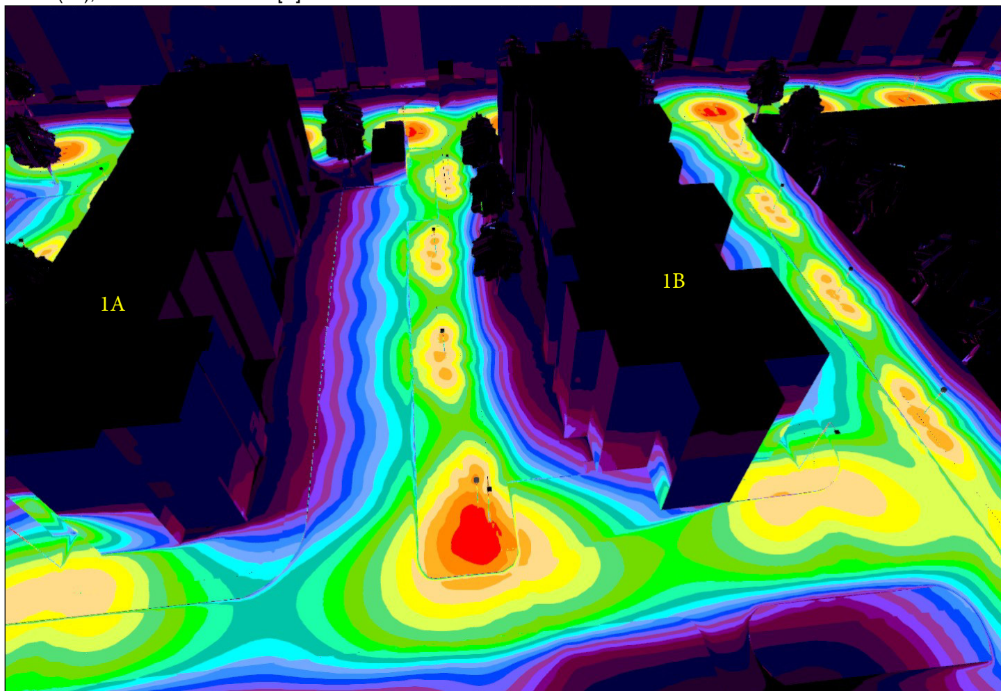
Site 1 (39), Illuminance values in [lx]
